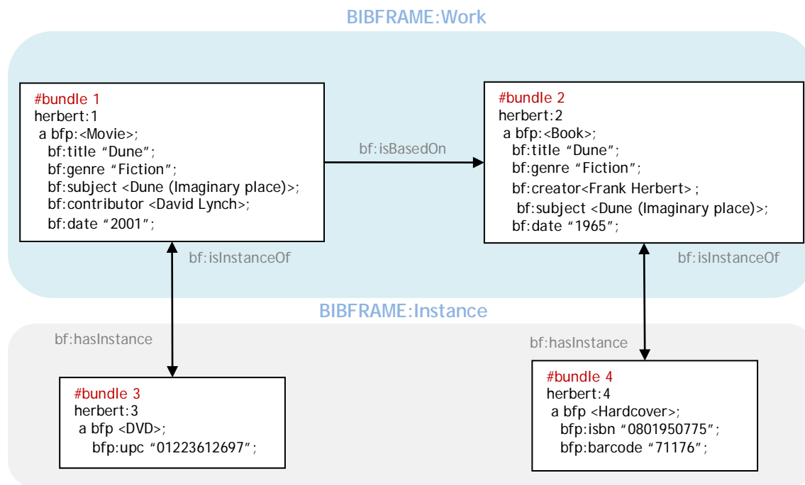
Figure 3.1. A schematic representation of BIBFRAME descriptions for Frank Herbert's 'Dune'
