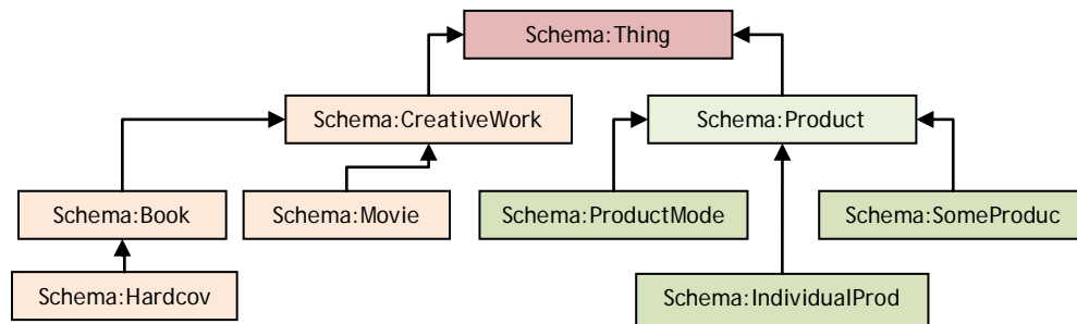
Figure 2.3. Schema.org CreativeWork and Product ontologies
